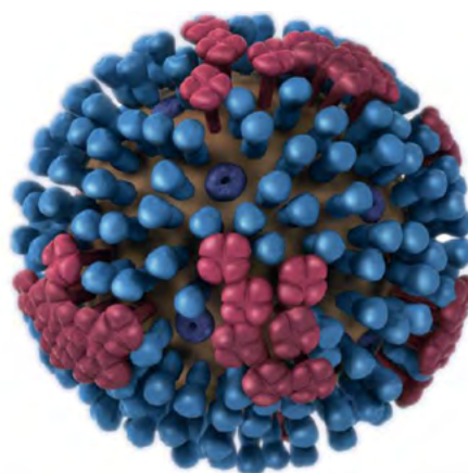
Gripas vīrusa 3D modelis. Avots: CDC/Dan Higgins/Science Source
